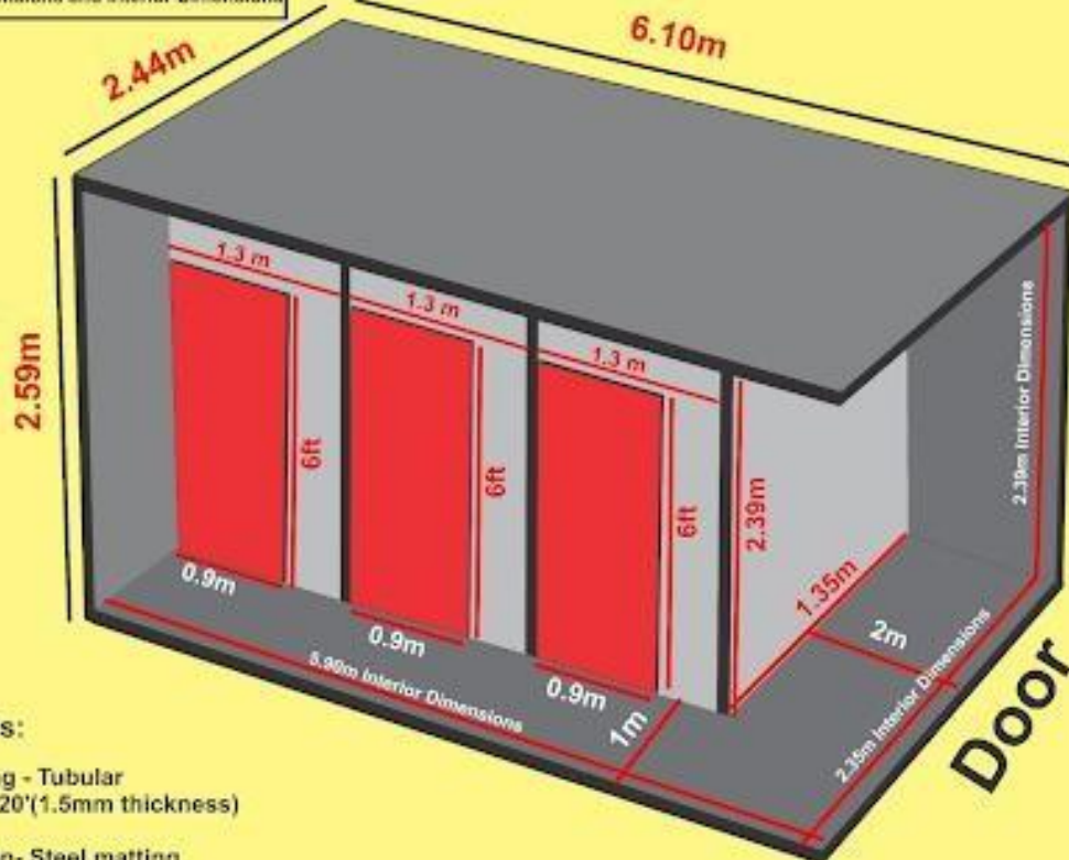
Container Van Exterior Dimensions and Interior Dimensions
